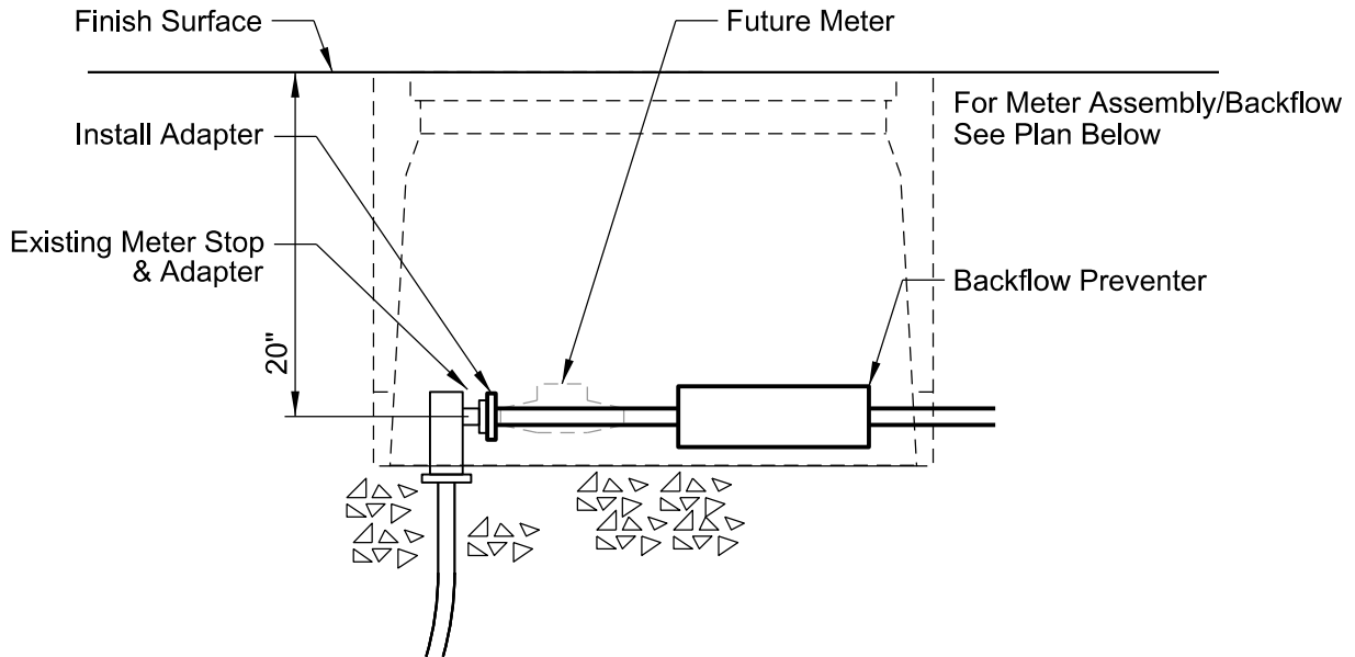
SERVICE LINE ASSEMBLY
