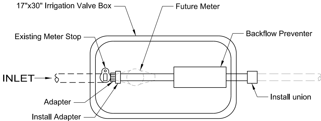
METER/BACKFLOW ASSEMBLY
